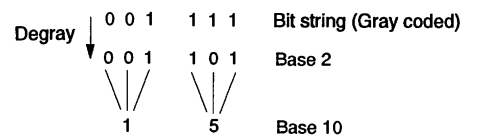
Fig. 2. Bit-string encoding of multiple real-valued parameters. An arbitrary string of six bits is interpreted in the following steps: (i) segment the string into two regions with the first three bits reserved for x and the second three bits for y ; (ii) interpret each three-bit substring as a Gray code and map back to the corresponding binary code (see Table 1); (iii) map each three-bit substring from its binary code to its decimal equivalent; (iv) substitute the two decimal values for x and y in the fitness function F ; and (v) return F(x, y) as the fitness of the original string.
