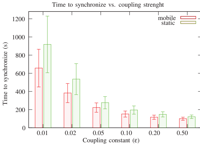
Fig. 7. Synchronization time for group of 50 simulated robots for coupling constants 0.01, 0.02, 0.05, 0.10, 0.20, 0.50. Each bar summarizes 100 runs and error bars denote the standard deviation. The density was 6 robots/m 2 .
