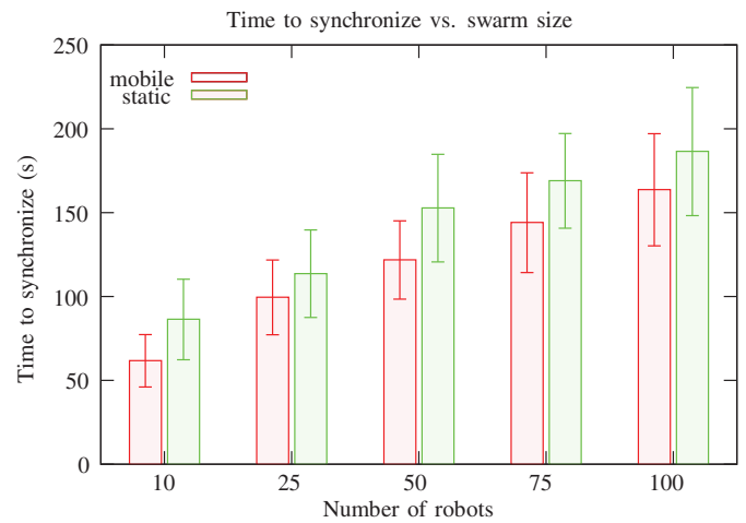
Fig. 5. Synchronization time for groups of 10 to 100 simulated robots. Each bar summarizes 100 runs and error bars denote the standard deviation. The density was 8 robots/ m^2 and a coupling constant of \epsilon = 0.1 was used in all runs.
