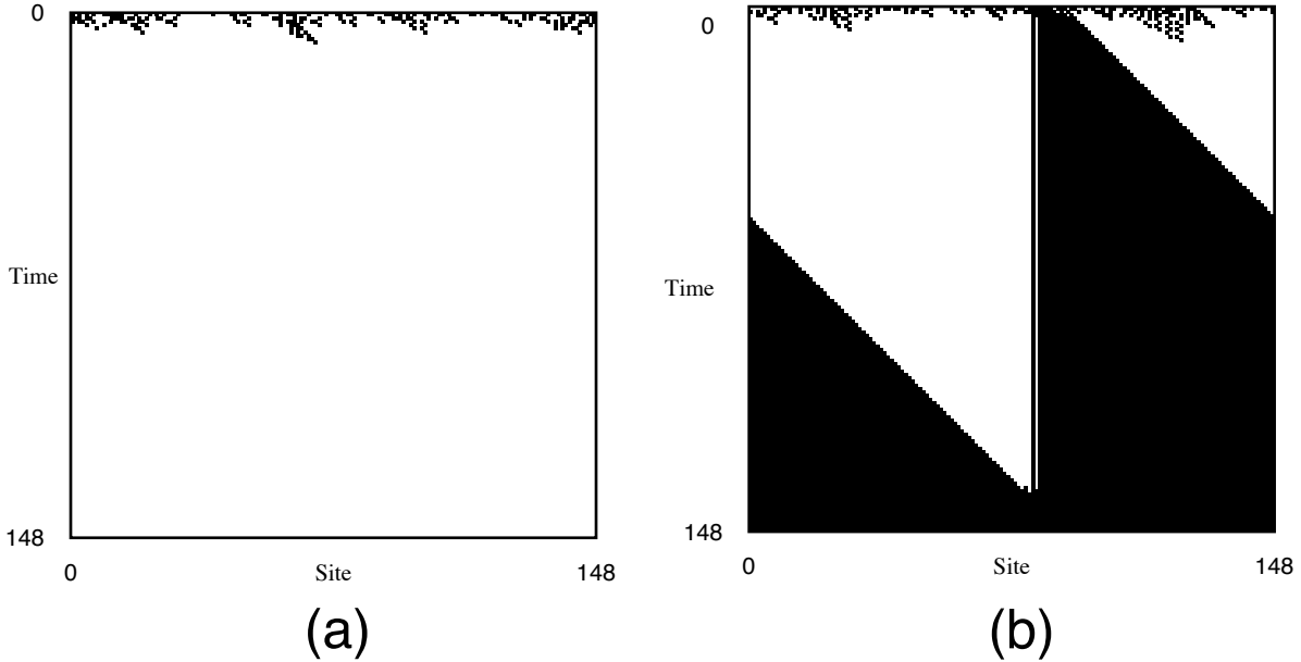
Figure 6: Two spacetime diagrams for an Epoch 4 rule with \lambda \approx 0.38 that implements Strategy 1. In (a), \rho_0 \approx 0.41 and in (b), \rho_0 \approx 0.52 .
